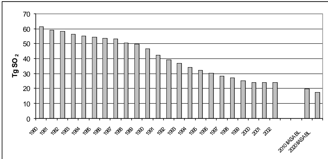
Figure I. Trends in sulphur emissions in the EMEP area (1980-2002, 2010, 2020)
