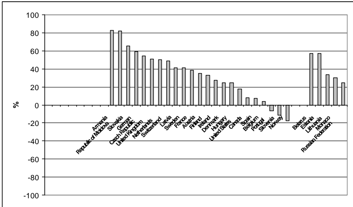
Figure IX. Reductions in emissions of non-methane volatile organic compounds in the ECE region (1990-2002) (based on the latest data available). Signatories to the 1999 Gothenburg Protocol are on the left. Only countries that have reported national total emission data, including main sources, for both 1990 and 2002 are listed here.
