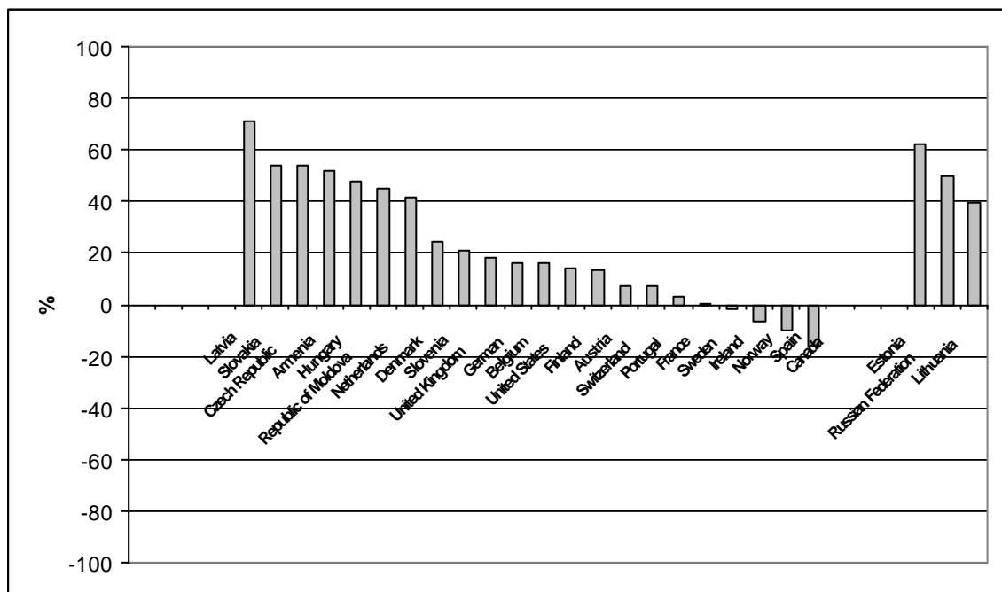
Figure VIII. Ammonia emission reductions in the ECE region (1990-2002) (based on the latest data available). Signatories to the 1999 Gothenburg Protocol are on the left. Only countries that have reported national total emission data, including main sources, for both 1990 and 2002 are listed here.
